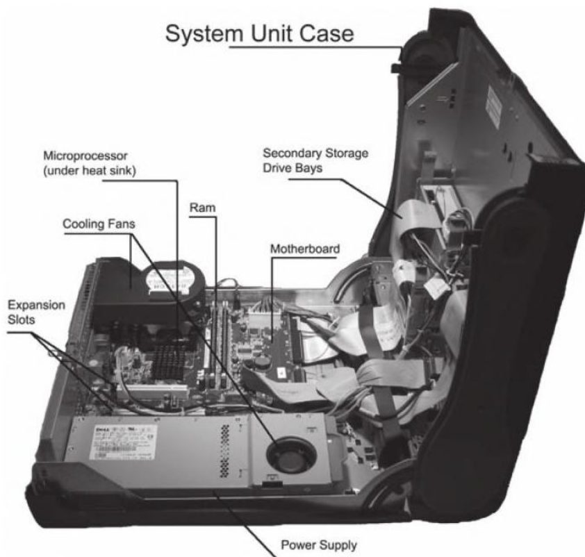
Figure 3.2 System unit.
