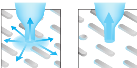
Figure 3.13 Pits scatter light and lands reflect light.
